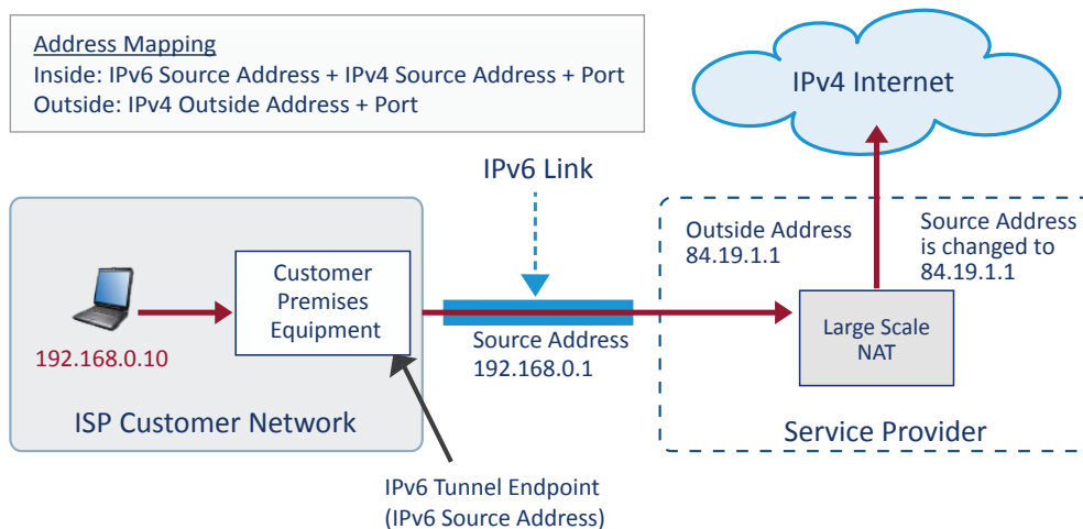
Figure 1 Dual Stack Lite tunnels IPv4 packets over IPv6 between the user and the Large Scale NAT
